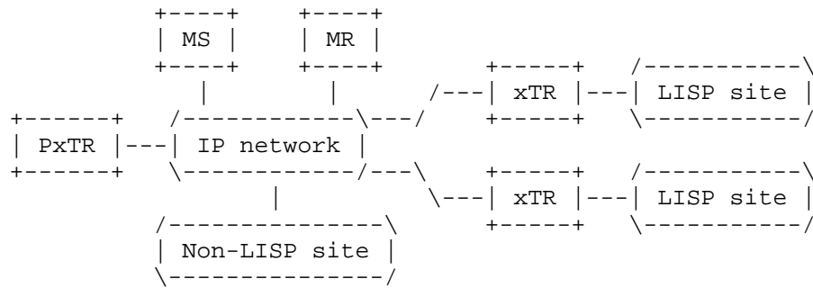
An Example of a LISP Deployment
